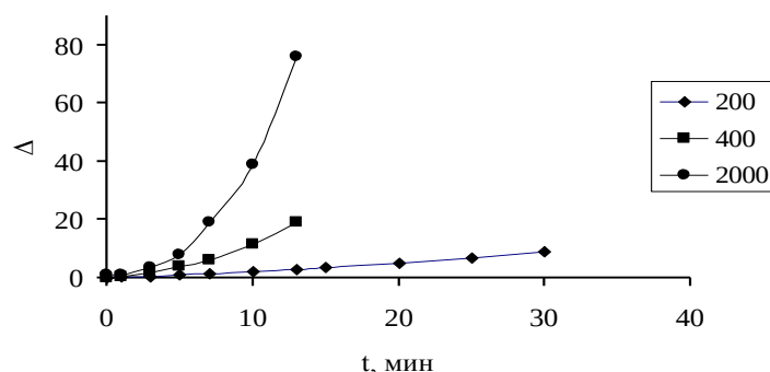
Fig. 13. Kinetics of heteroadagulation particles on polyester-fabric. S-curves similar to autocatalytic mode
